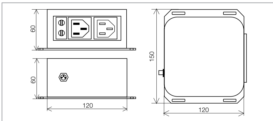
Fig. 2 Dimensional drawing, dimensions in mm
