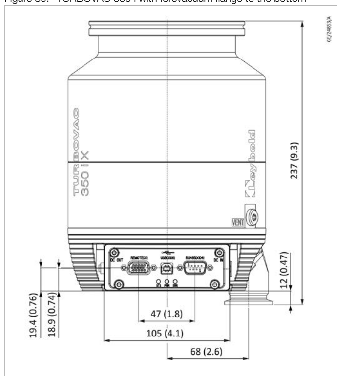
Figure 30. TURBOVAC 350 i with forevacuum flange to the bottom
