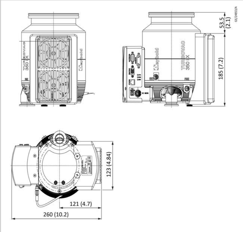
Figure 28. TURBOVAC 350 i(X) with radial air cooling
