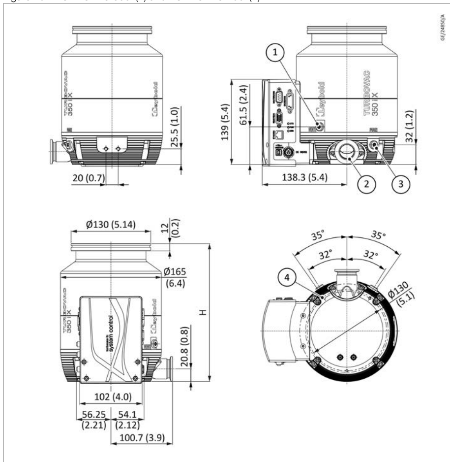
Figure 25. TURBOVAC 350 i(X) and TURBOVAC 450 i(X)
