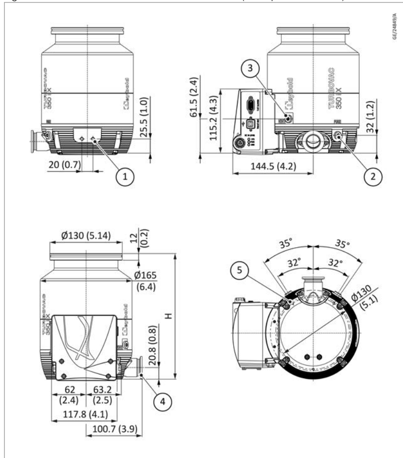
Figure 24. TURBOVAC 350 i and TURBOVAC 450 i (with optional interface)
