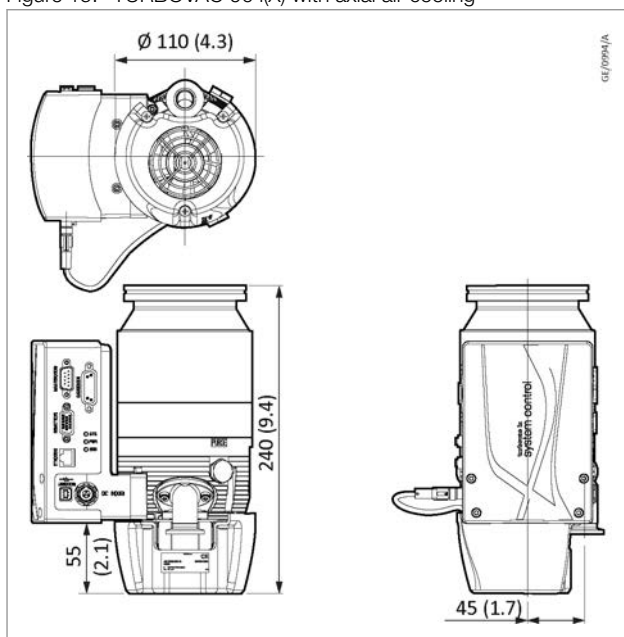
Figure 15. TURBOVAC 90 i(X) with axial air cooling
