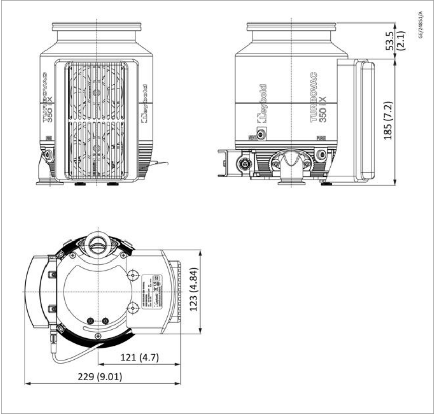
Figure 26. TURBOVAC 350 i with radial air cooling
