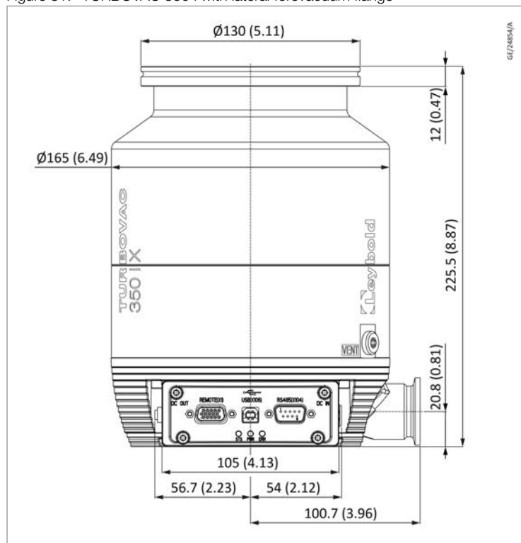
Figure 31. TURBOVAC 350 i with lateral forevacuum flange
