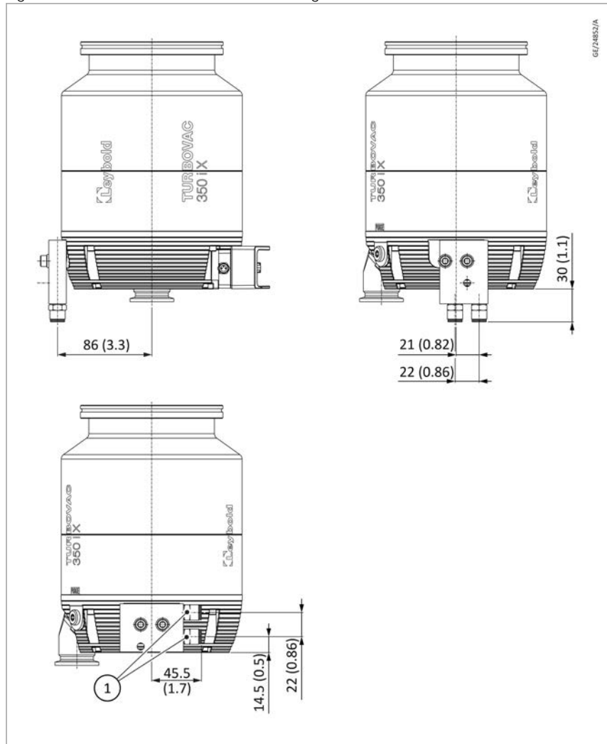
Figure 27. TURBOVAC 350 i with water cooling
