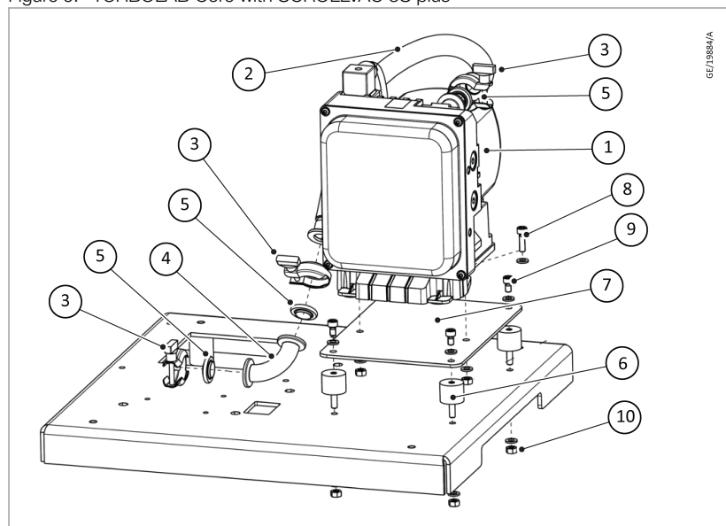
Figure 9. TURBOLAB Core with SCROLLVAC 3S plus
