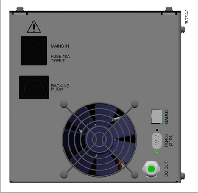
Figure 5. Rear panel
