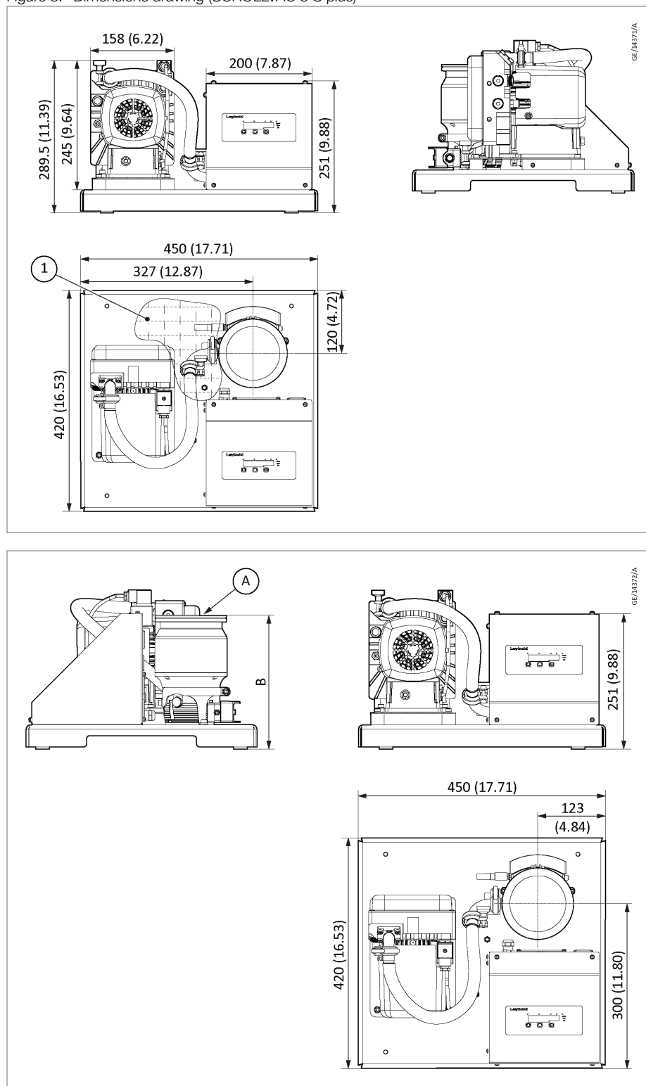
Figure 3. Dimensions drawing (SCROLLVAC 3 S plus)
