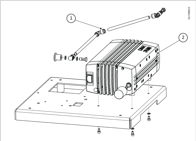
Figure 8. TURBOLAB Core with DIVAC backing pump
