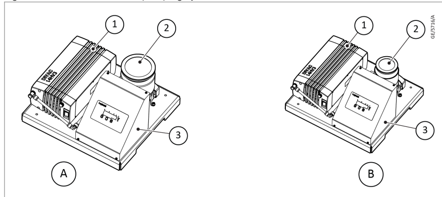
A. TV250i with DIVAC 1.4
