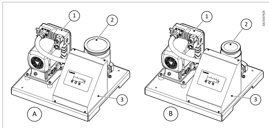
A. TV250i with SCROLLVAC 3 S plus
