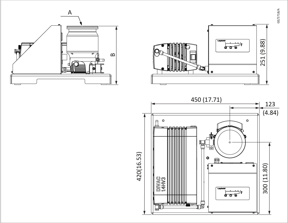
Figure 2. Dimensions drawing
