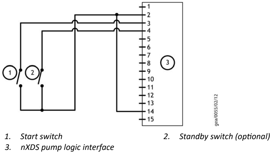
Figure 10 Logic interface connections - parallel control
