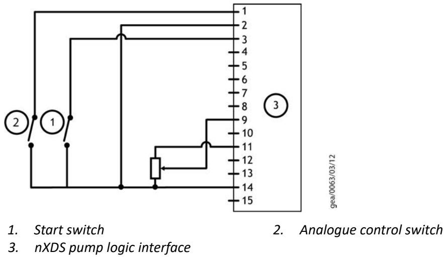
Figure 11 Logic interface connections - analogue speed control
