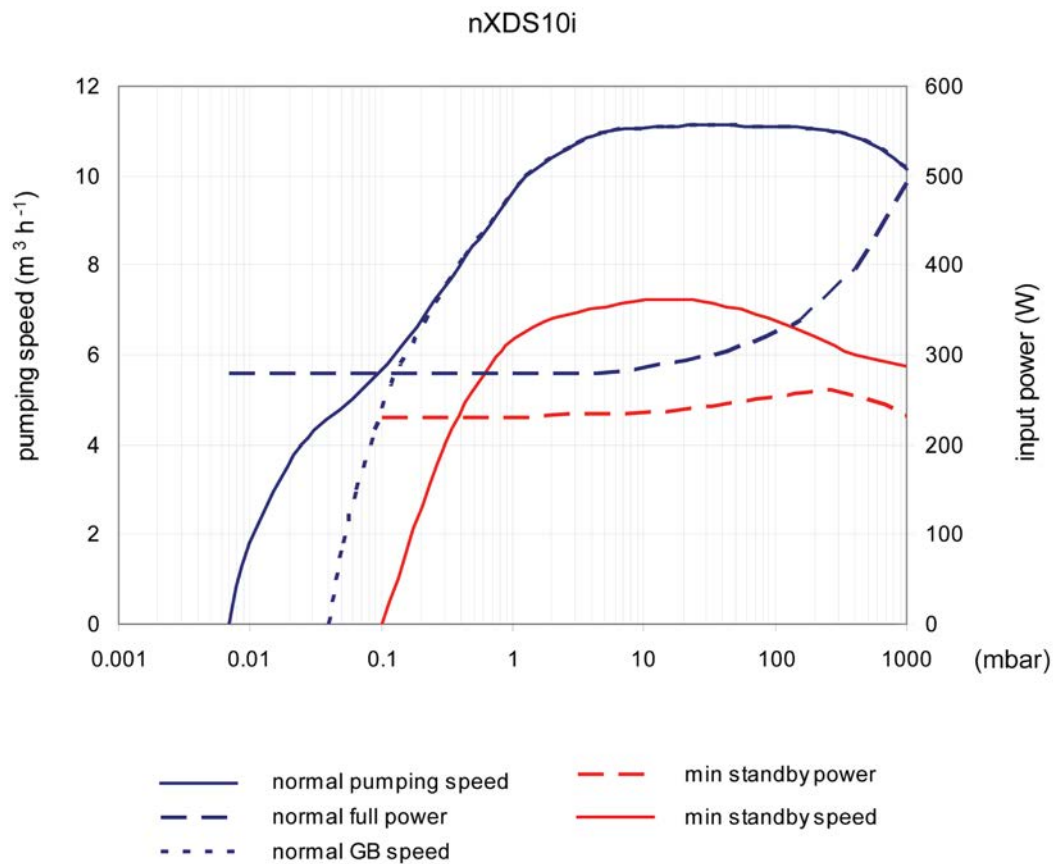
Figure 4 nXDS10i Performance characteristics
