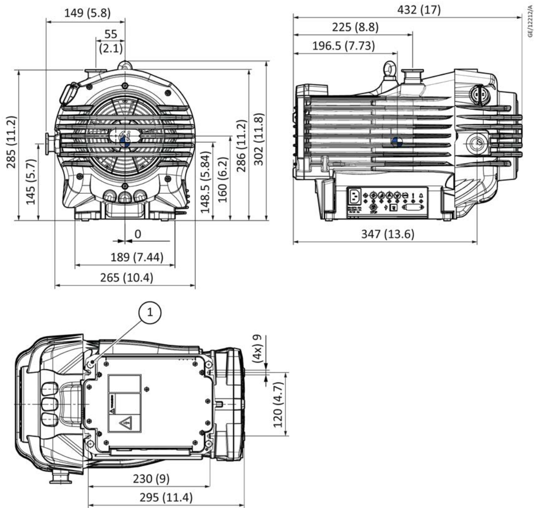
Figure 8 Installation drawing
