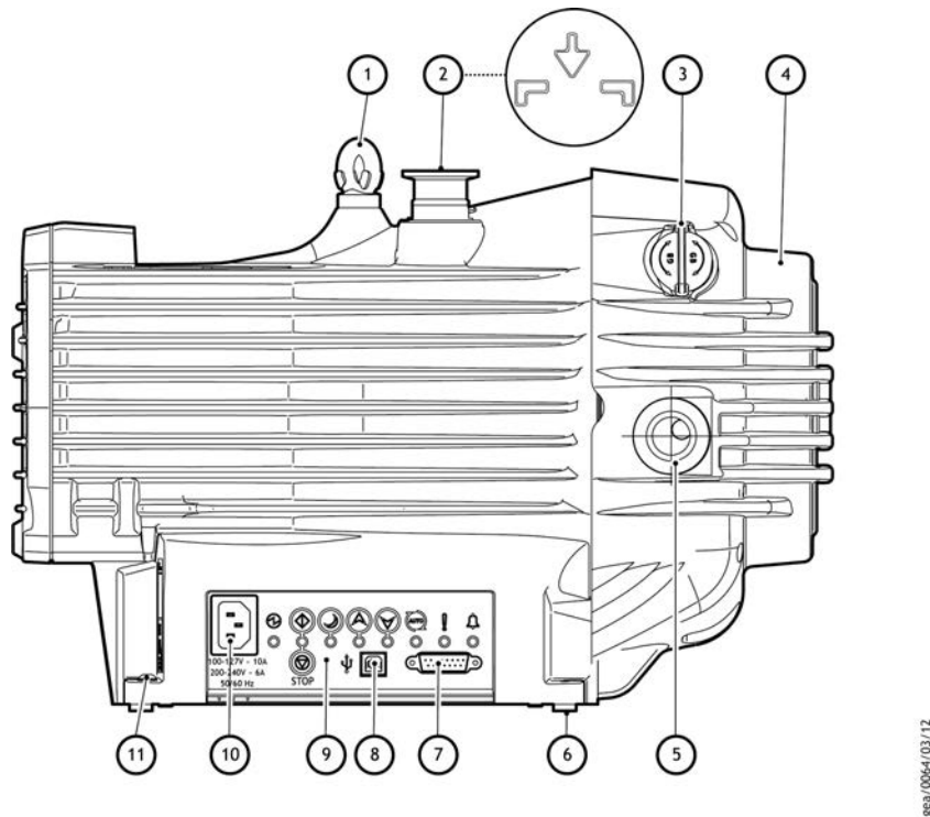
Figure 1 nXDS scroll pump
