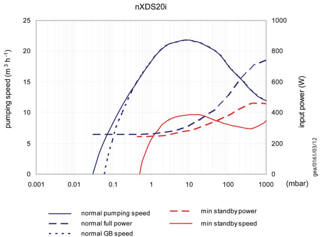
Figure 6 nXDS20i Performance characteristics
