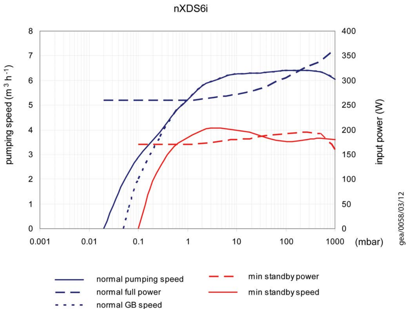
Figure 3 nXDS6i Performance characteristics
