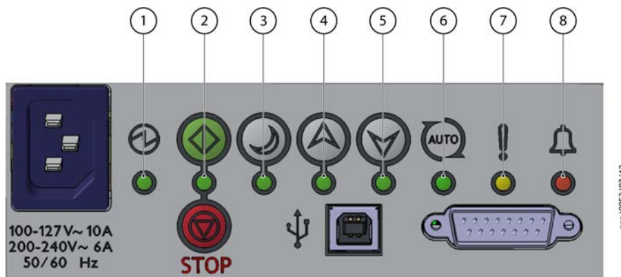
Figure 7 LED indicators
