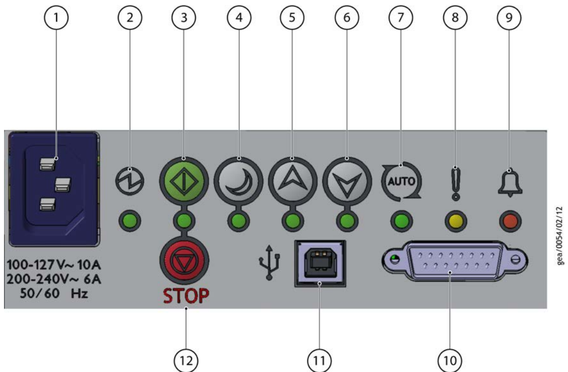
Figure 9 User interface panel
